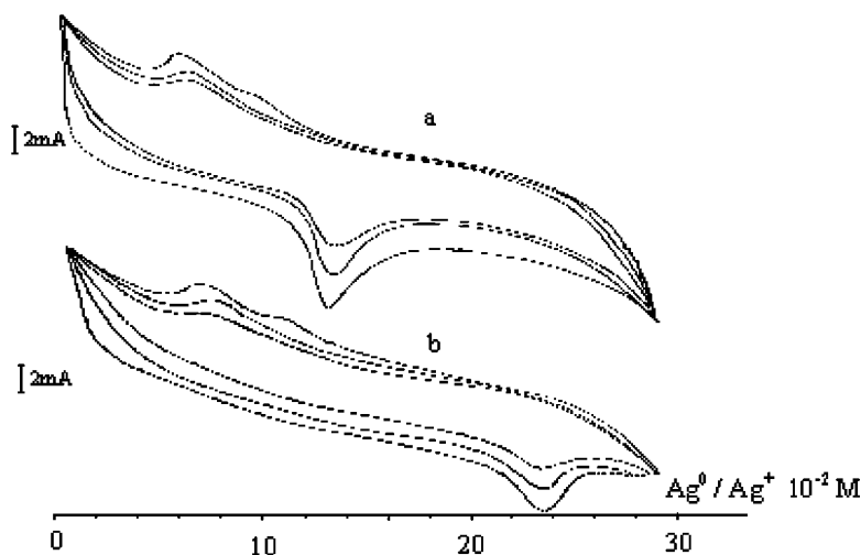
FIGURE 1 The cyclic voltammograms of thiophene, (a) on bare Pt electrode and (b) on PAA coated electrode.
