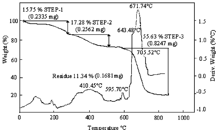
FIGURE 7 TGA thermogram of PTh-PAA composite film.
