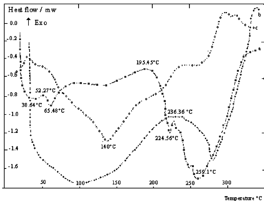
FIGURE 2 DSC thermogram of: (a) polyacrylamide, (b) polythiophene, (c) PTh-PAA composite film.
