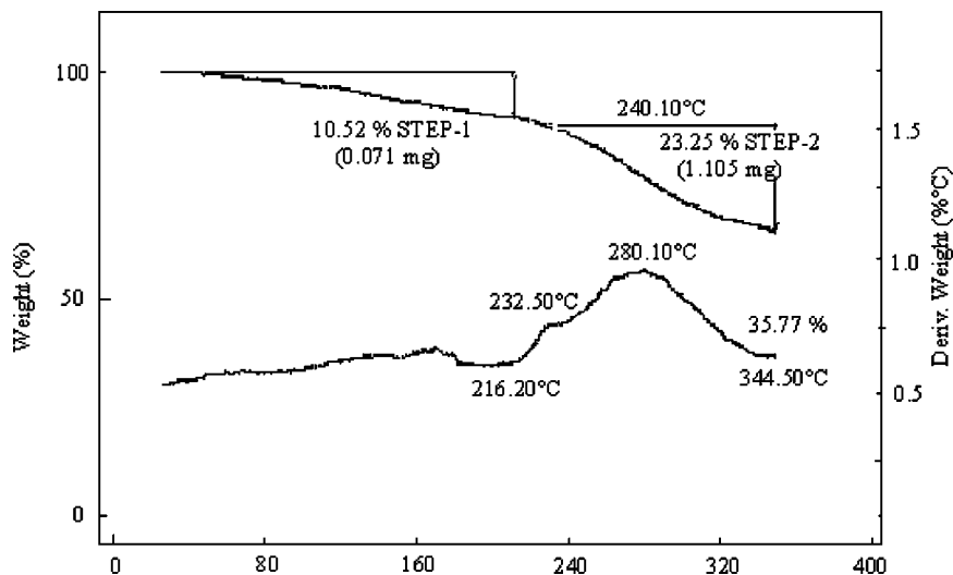
FIGURE 5 TGA thermogram of polyacrylamide.
