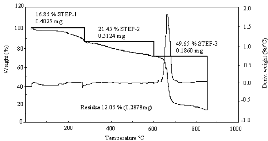
FIGURE 6 TGA thermogram of polythiophene.
