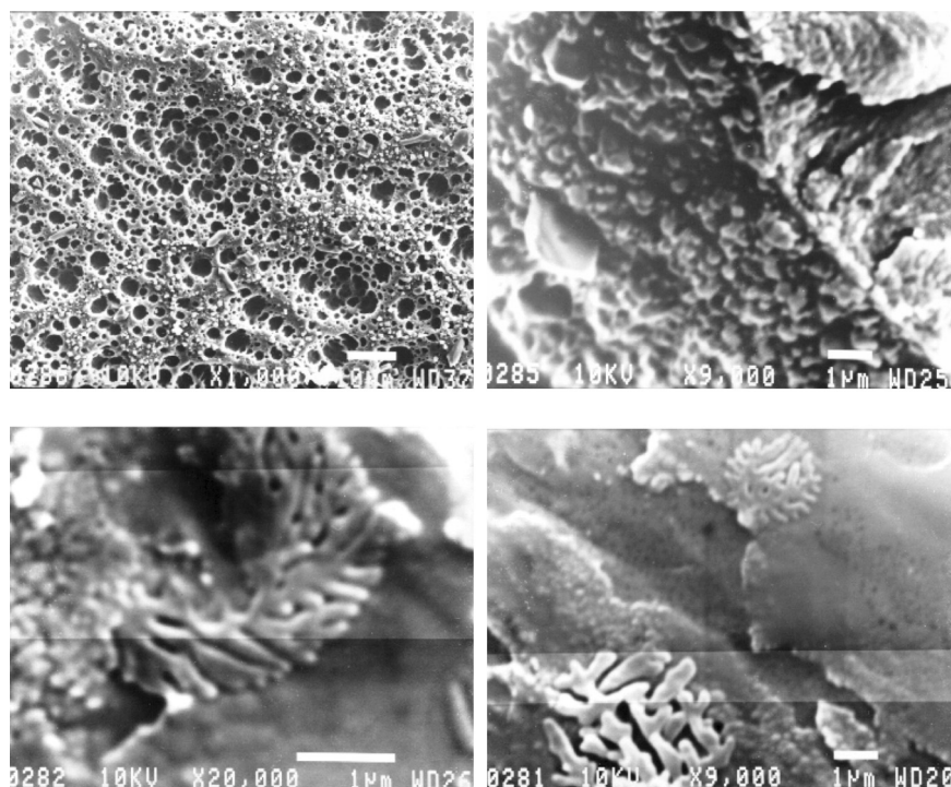
FIGURE 4 SEM pictures of (a) PTh solution side, (b) PTh-PAA film electrode side, (c) PTh-PAA film solution side, (d) PTh-PAA film solution side of washed film.
