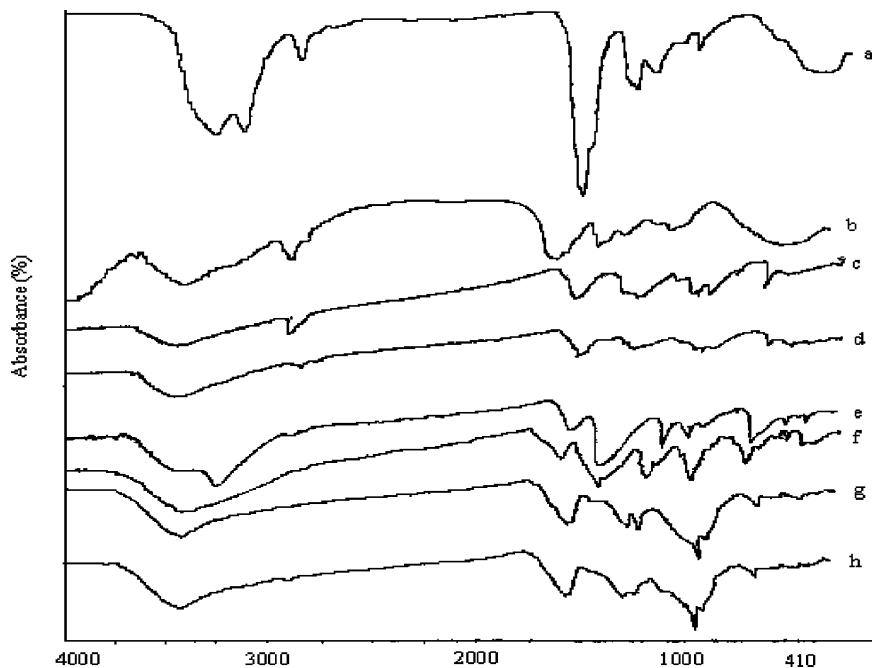
FIGURE 3 IR spectra of PTh-PAA films (a) 100% PAA, (b) 66.65% PAA–33.35% PTh, (c) 45.03% PAA–54.97% PTh, (d) 36.71% PAA–64.29% PTh, (e) 26.08% PAA–73.92% PTh, (f) 19.35% PAA–81.65% PTh, (g) 10.25% PAA–89.75% PTh, (h) 100% PTh.
